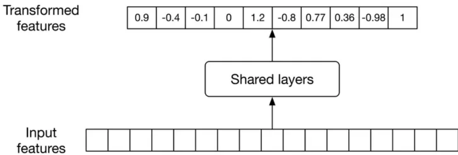
Figure 5.10: Shared layers
