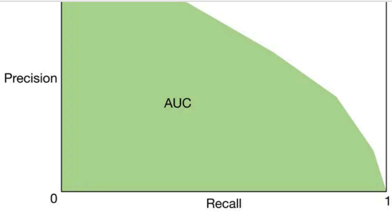
Figure 5.18: PR curve
