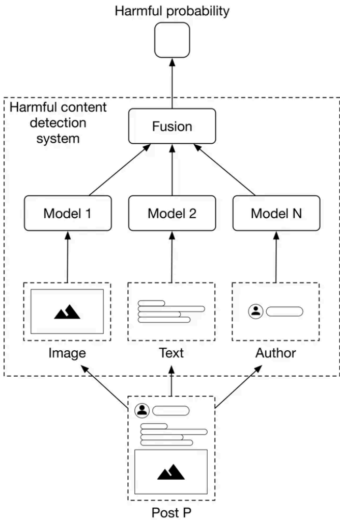
Figure 5.4: Late fusion
