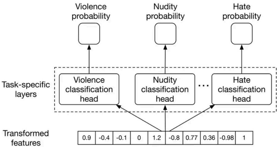
Figure 5.11: Task-specific layers
