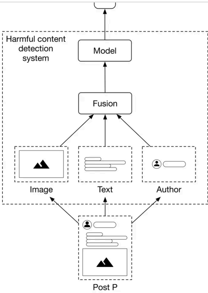
Figure 5.5: Early fusion
