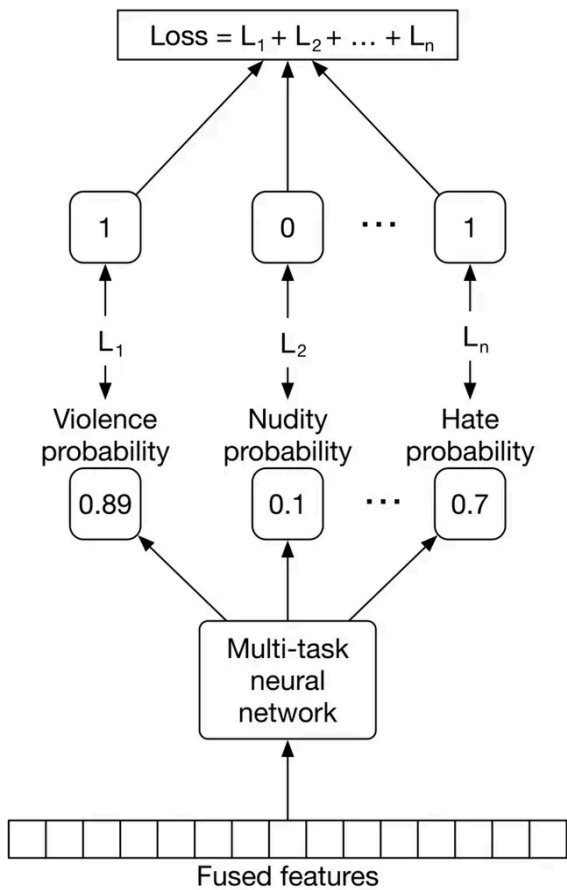
Figure 5.17: Model training
